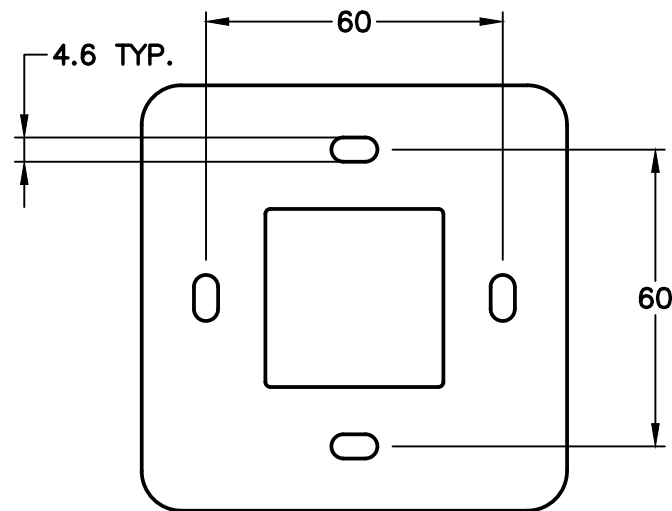
MOUNTING DIMENSIONS (SHOWN WITHOUT COVER)
