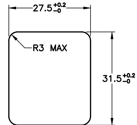
MOUNTING DIMENSIONS
