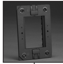
79170X45-N Mounting Frame. Fits on USA 2x4 Boxes. Accepts 22.5mm, 45mm & 67.5mmx45mm Devices.
