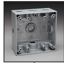
79430 Surface Mount Standard American 4x4 Wall Box. Cast Aluminum. 1/2 inch NPT Entries. Use with 4x4 Mounting Frames and Wall Plates.
