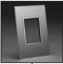
79185X45-N Finish Plate. Brushed Stainless Steel. Fits 79170X45-N Mounting Frame. Opening Size 67.5x45mm.
