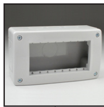
680604X45 Surface Mount Box. 90mmx45mm Opening. Gray. Accepts 22.5mm, 45mm & 67.5mmx45mm Devices.
