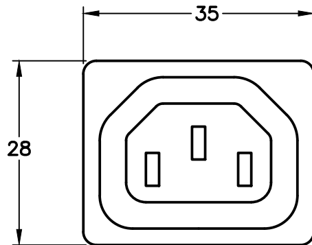
IEC 60320 C-13 FRONT VIEW
